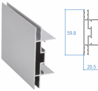
Size(H*W*wt) : 59.8 × 21 × 1.4
