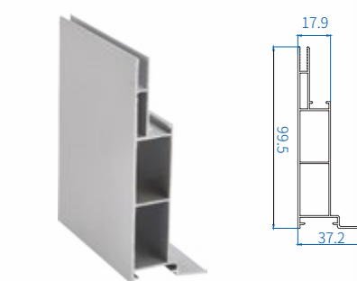
Size(H*W*wt) : 99.6 × 37.2 × 1.4
