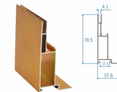
Size(H*W*wt) : 78.6 × 38.6 × 1.4
